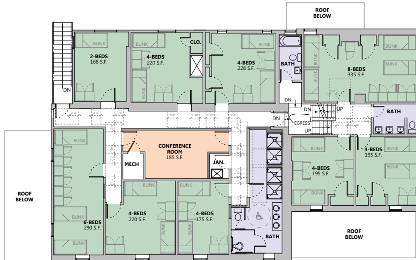
SECOND FLOOR SCHEME A 1/8" = 1'-0"
