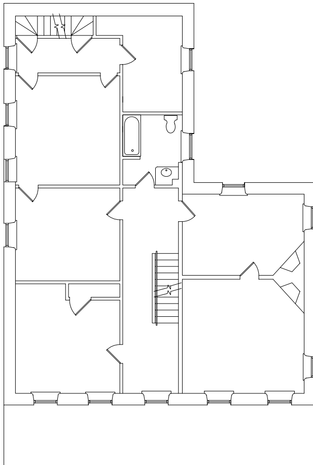
2nd Floor
